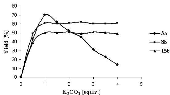
Figure 2. Plot of the yield [%] obtained in the condensation of 2-chlorobenzoic acids derivatives with a primary amine ( 3a ), secondary cyclic amine ( 8b ) or secondary acyclic amine ( 15b ) as a function of K_2CO_3 equivalents.
