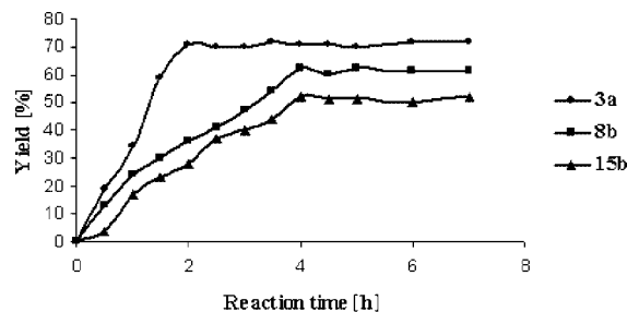
Figure 1. Plot of the yield [%] obtained in the condensation of 2-chlorobenzoic acid derivatives with a primary amine ( 3a ), secondary cyclic amine ( 8b ) or secondary acyclic amine ( 15b ) as a function of reaction time [h].
