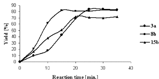
Figure 3. Plot of yield [%] obtained in the condensation of 2-chlorobenzoic acid derivatives with a primary amine ( 3a ), secondary cyclic amine ( 8b ) or secondary acyclic amine ( 15b ) in the presence of ultrasonic irradiation as a function of reaction time [min].
