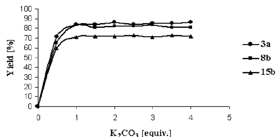
Figure 4. Plot of yield [%] obtained in the condensation of 2-chlorobenzoic acid derivatives with a primary amine ( 3a ), secondary cyclic amine ( 8b ) or secondary acyclic amine ( 15b ) in the presence of ultrasonic irradiation as a function of K 2 CO 3 equivalents.
